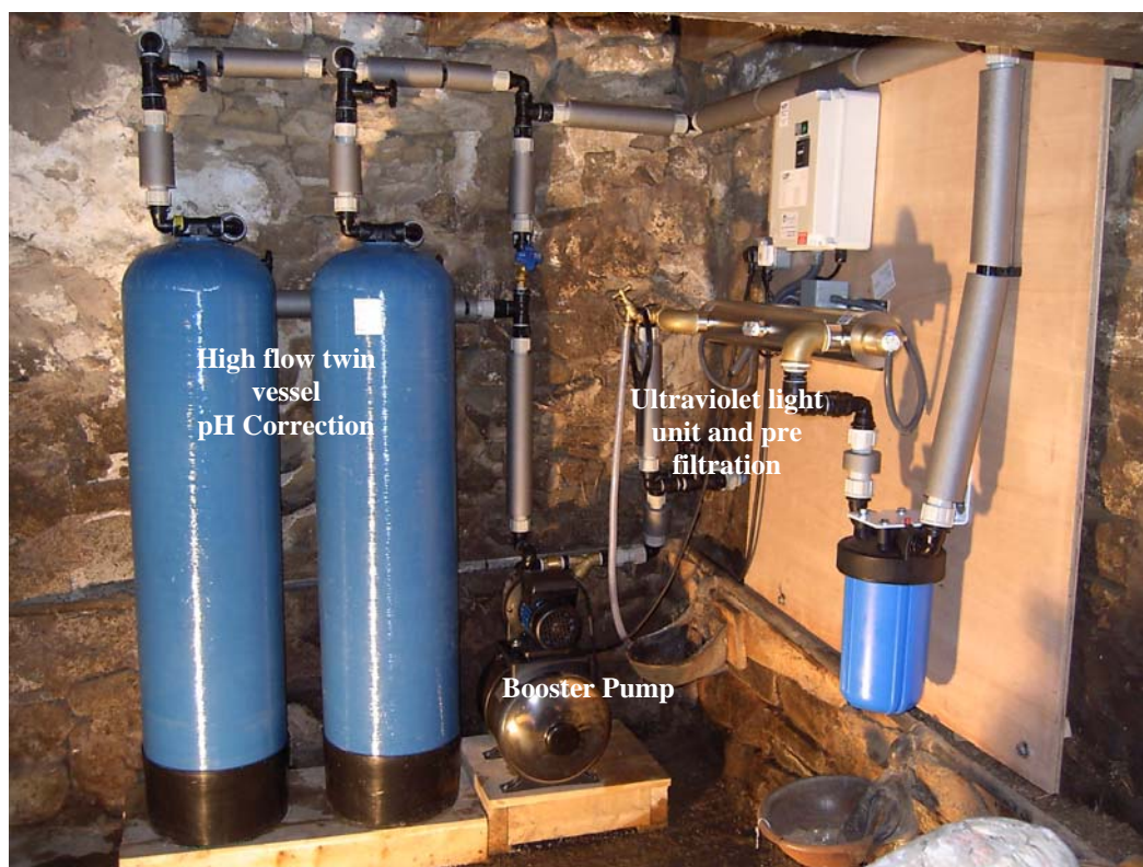
High flow, twin vessel pH corrector configuration
